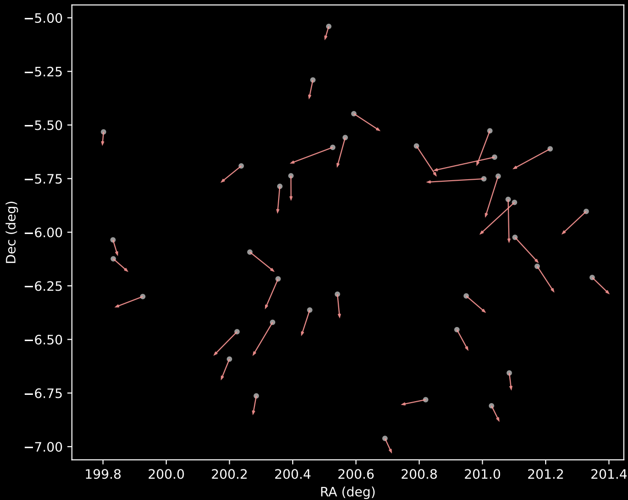
GALAH DR4 Cluster 7 Proper Motion Vectors (n=38)
