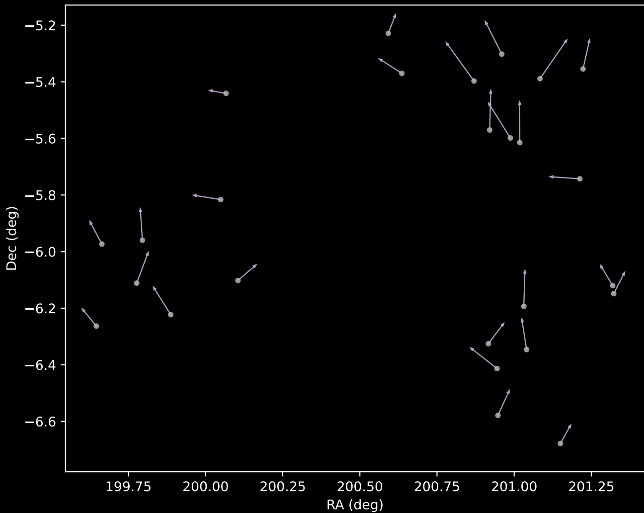
GALAH DR4 Cluster 9 Proper Motion Vectors (n=26)
