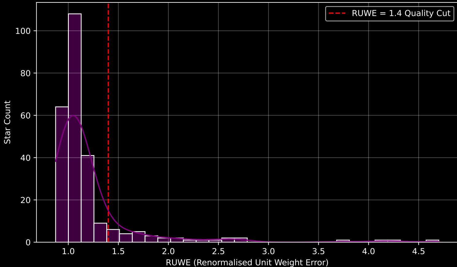
GALAH DR4 Field [9028] RUWE Distribution (n= 255)
