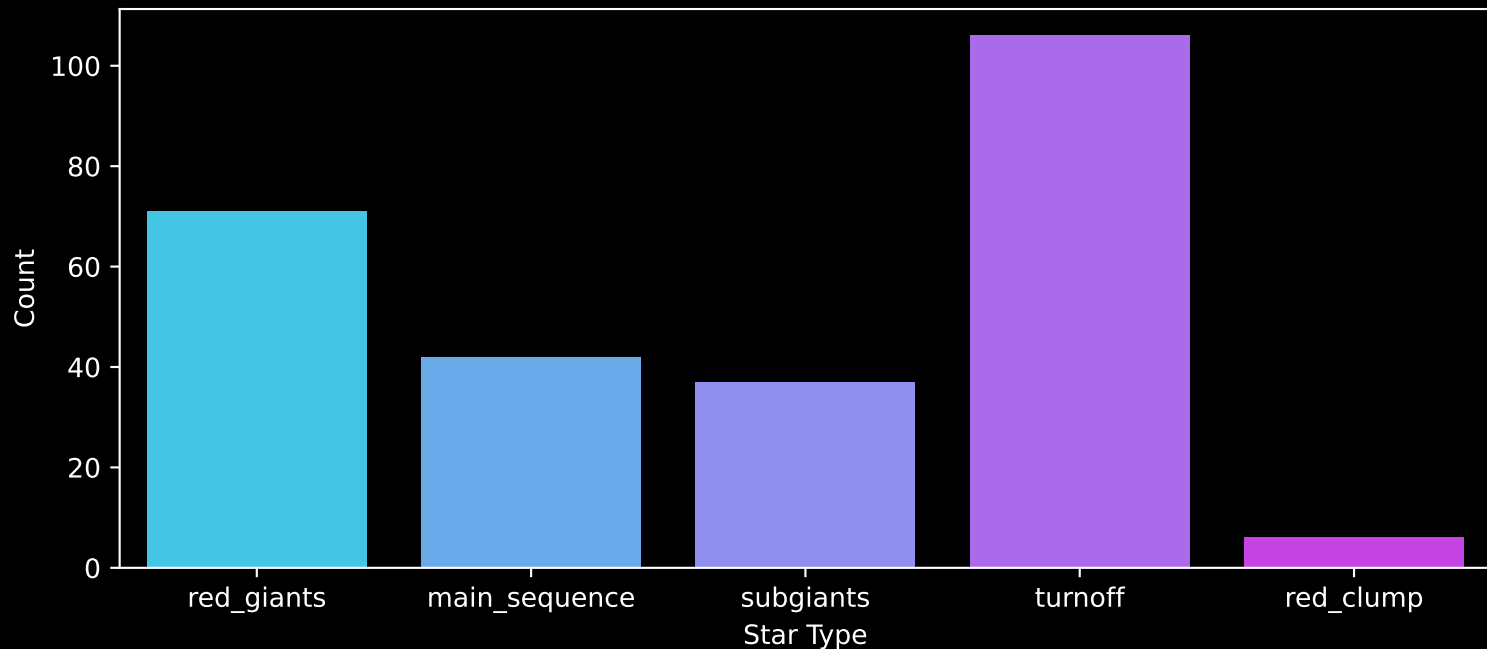
GALAH DR4 Field: [9028] Count plot of Star Type
